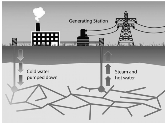
Photograph 3.11: Geothermal Energy
