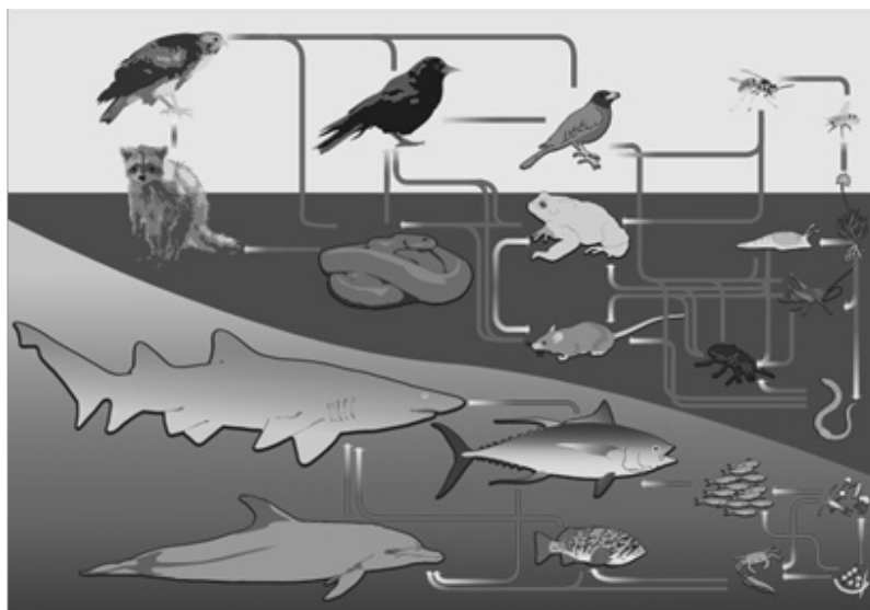
Photograph 1.9: Food Web
