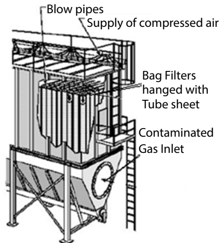
Figure 2.3: Typical pulse jet bag filters
