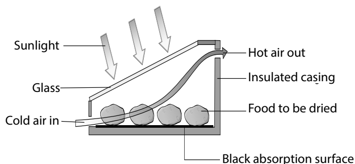
Photograph 3.4: Solar Dryer
