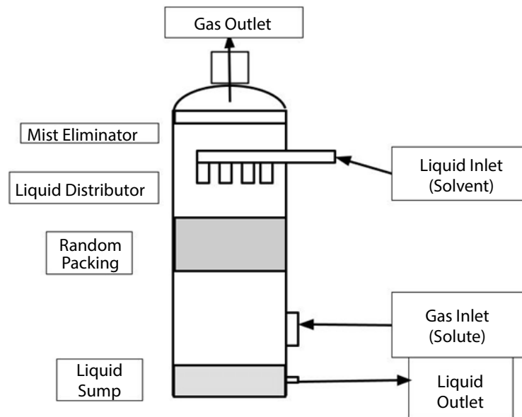
Figure 2.5: Packed-bed counter flow scrubber
