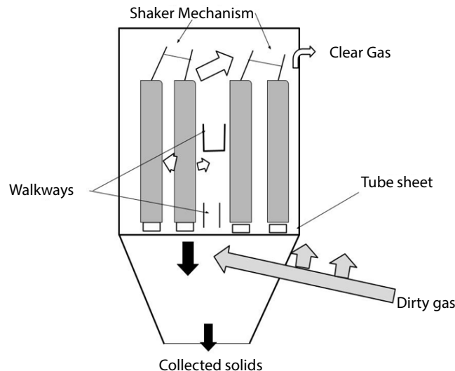
Figure 2.1: Typical shaker bag filters
