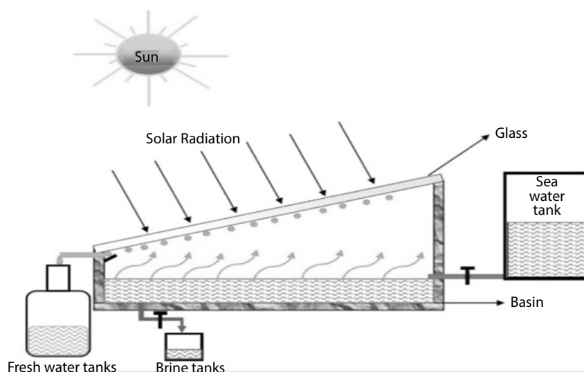
Photograph 3.5: Solar Stills
