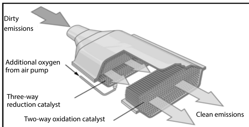
Figure 2.6: A schematic diagram of catalytic converter
