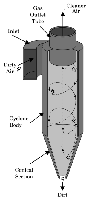
Figure 2.4: Typical Cyclone Separators
