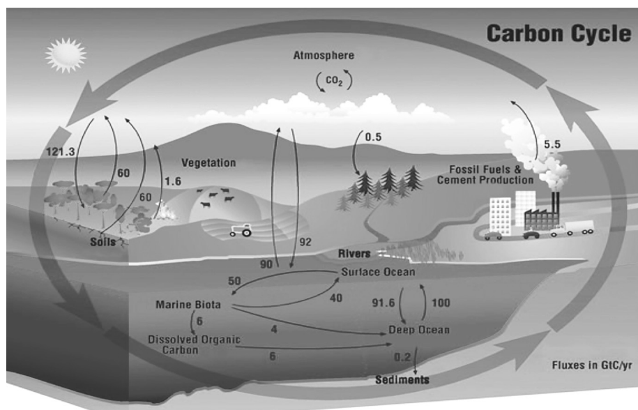
Photograph 1.10: Carbon Cycle
