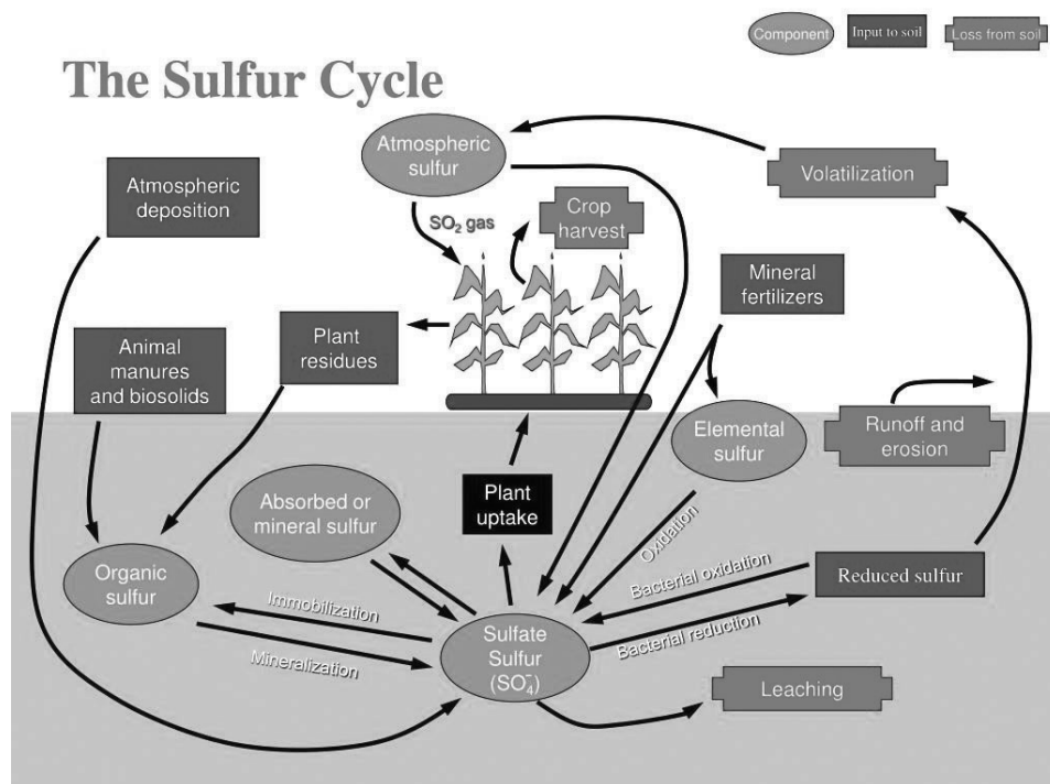
Photograph 1.12: Sulphur Cycle
