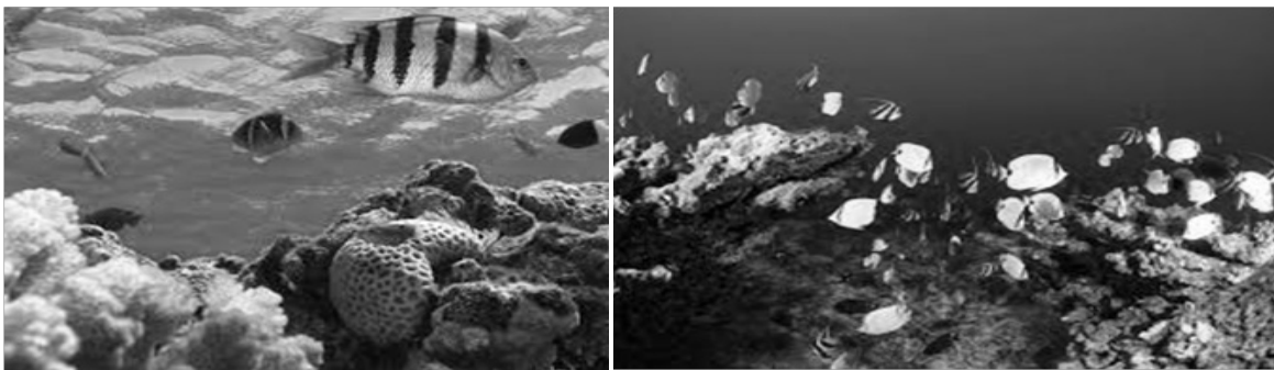
Photograph 1.3: Aquatic Ecosystem
