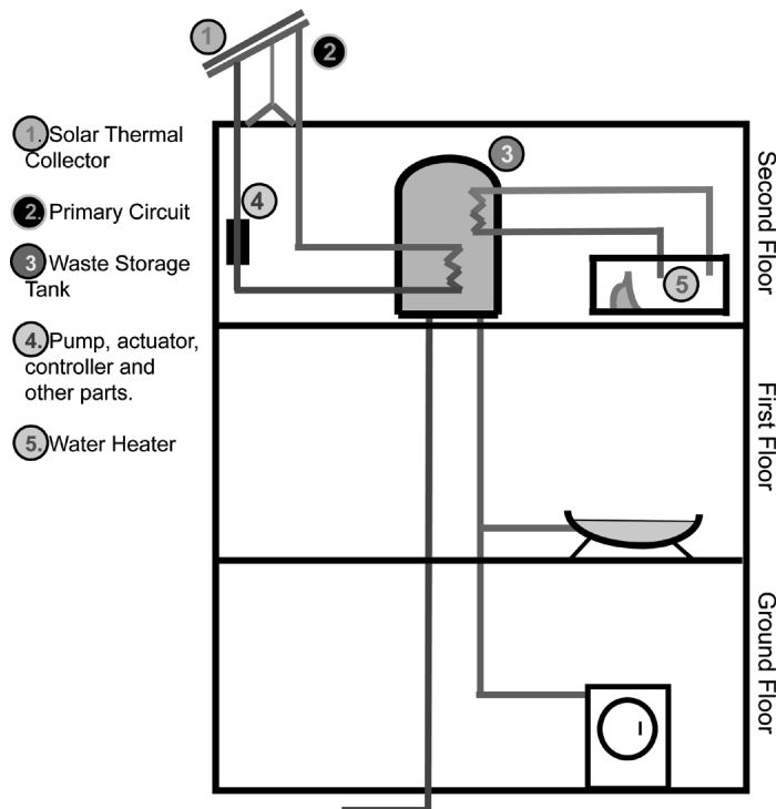
Figure 3.1: Solar Water Heater
